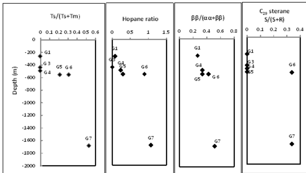
Fig. S1. Correlation with depth of biomarker parameters calculated on the base of cyclic structures.
